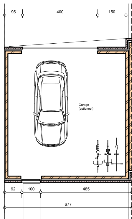
Garage
